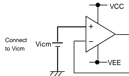
Figure 104. Example of application circuit for unused op-amp
