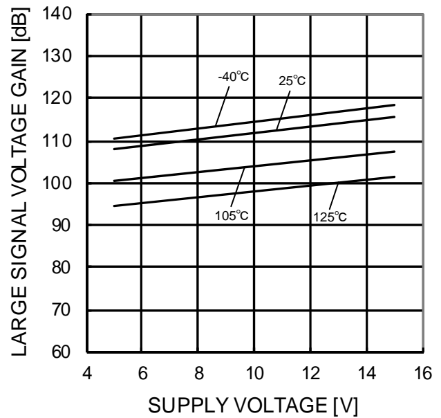
Figure 69. Large Signal Voltage Gain - Supply Voltage (RL=2kΩ)
