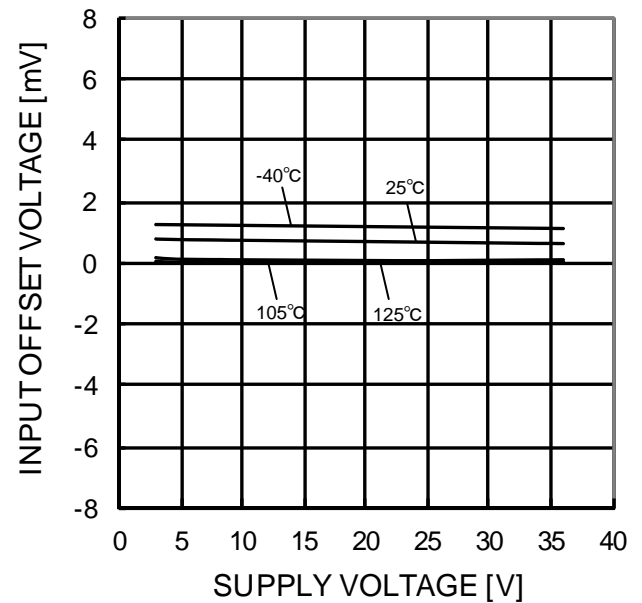
Figure 61. Input Offset Voltage - Supply Voltage (Vicm=0V, OUT=1.4V)
